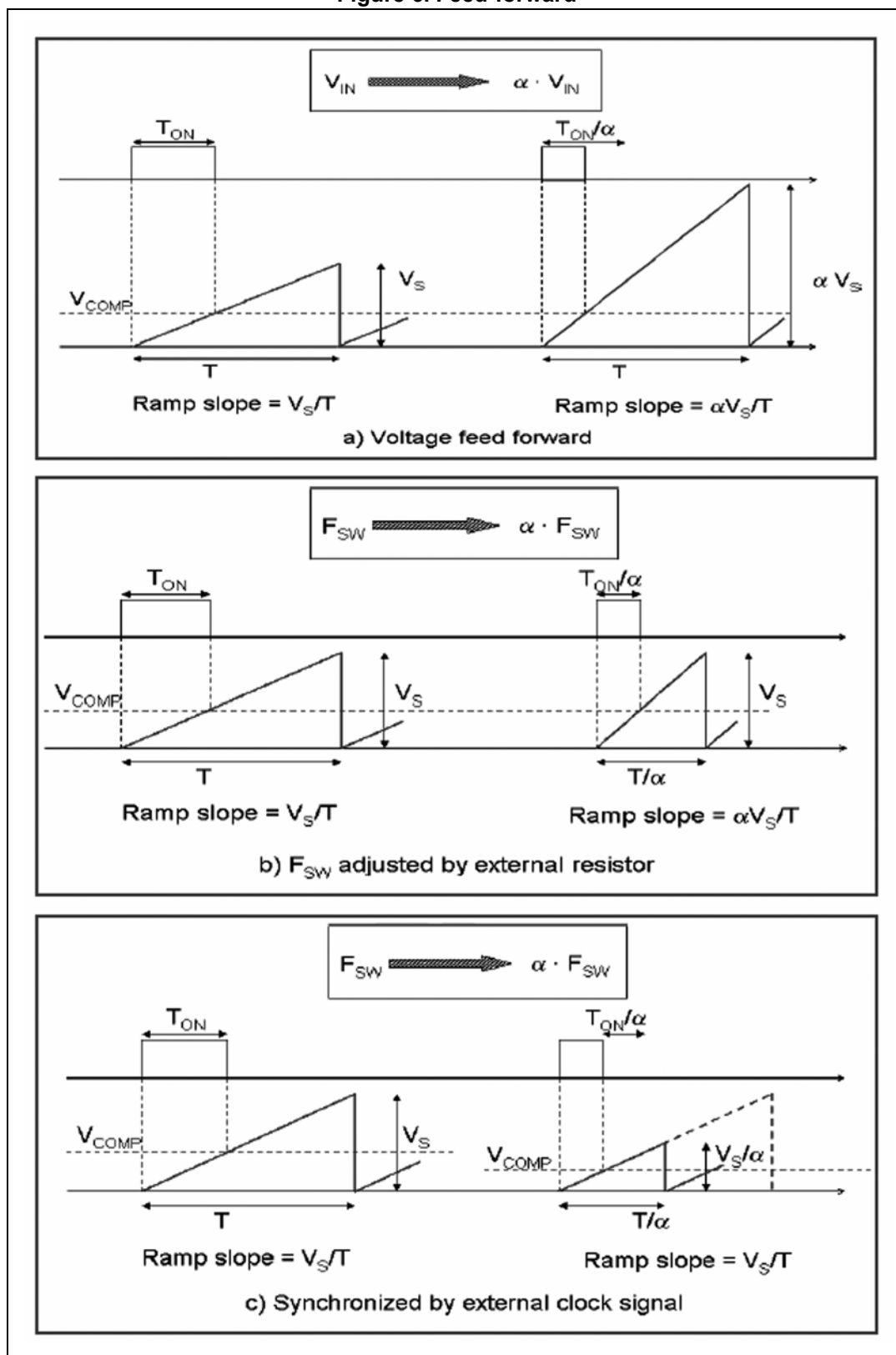
Figure 6. Feed-forward
