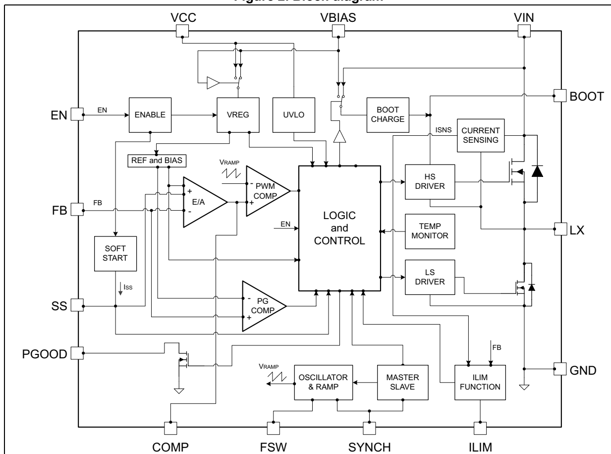
Figure 2. Block diagram
