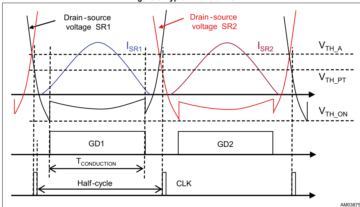
Figure 5. Typical waveforms
