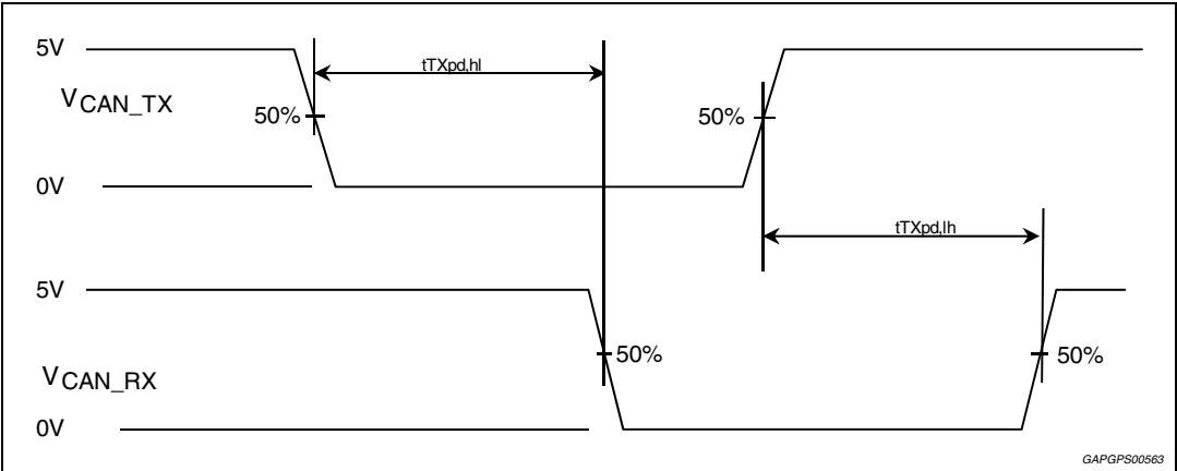
Figure 57. CAN transceiver switching waveforms
