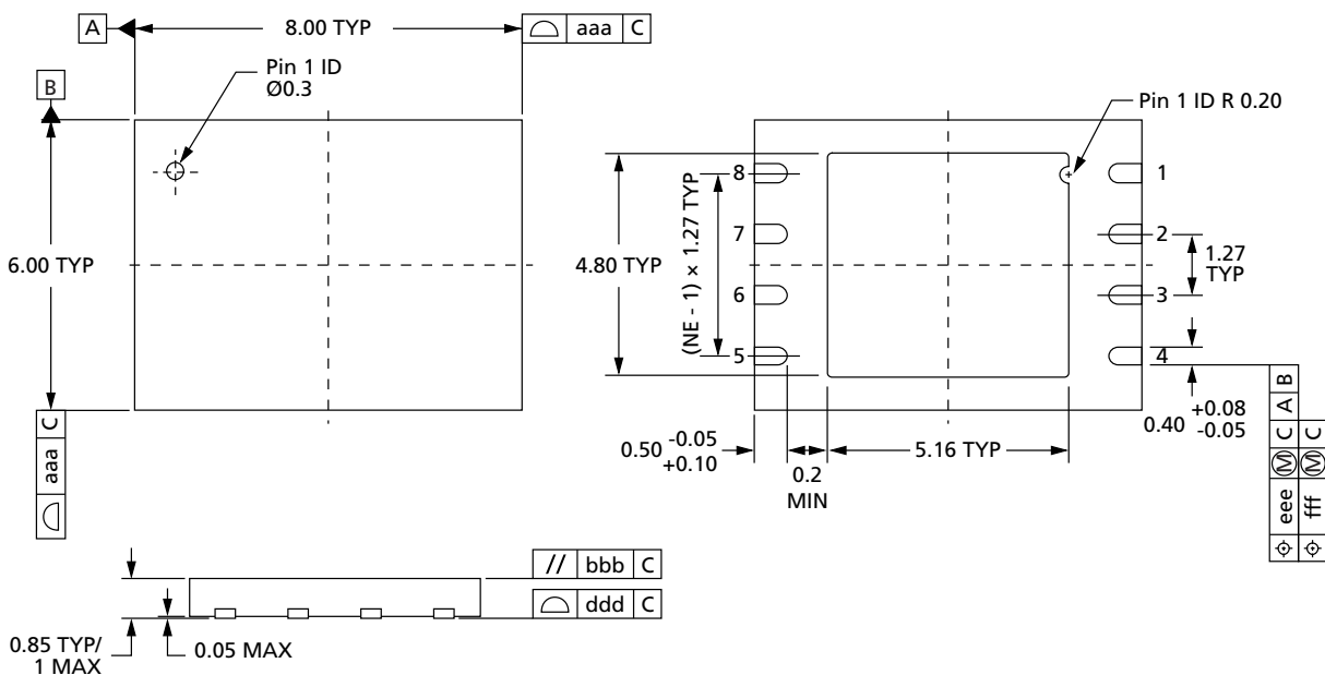
Figure 26: VFDFPN8 (MLP8) 8mm x 6mm – Package Code: ME
